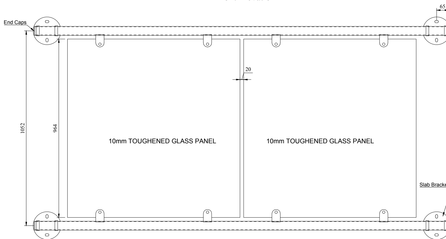
Front Elevation
