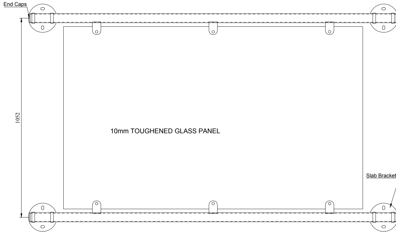
Front Elevation
