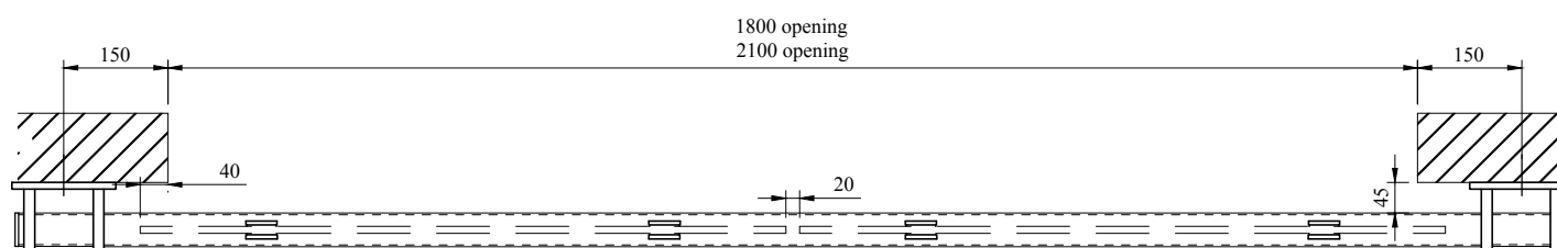
Plan View
