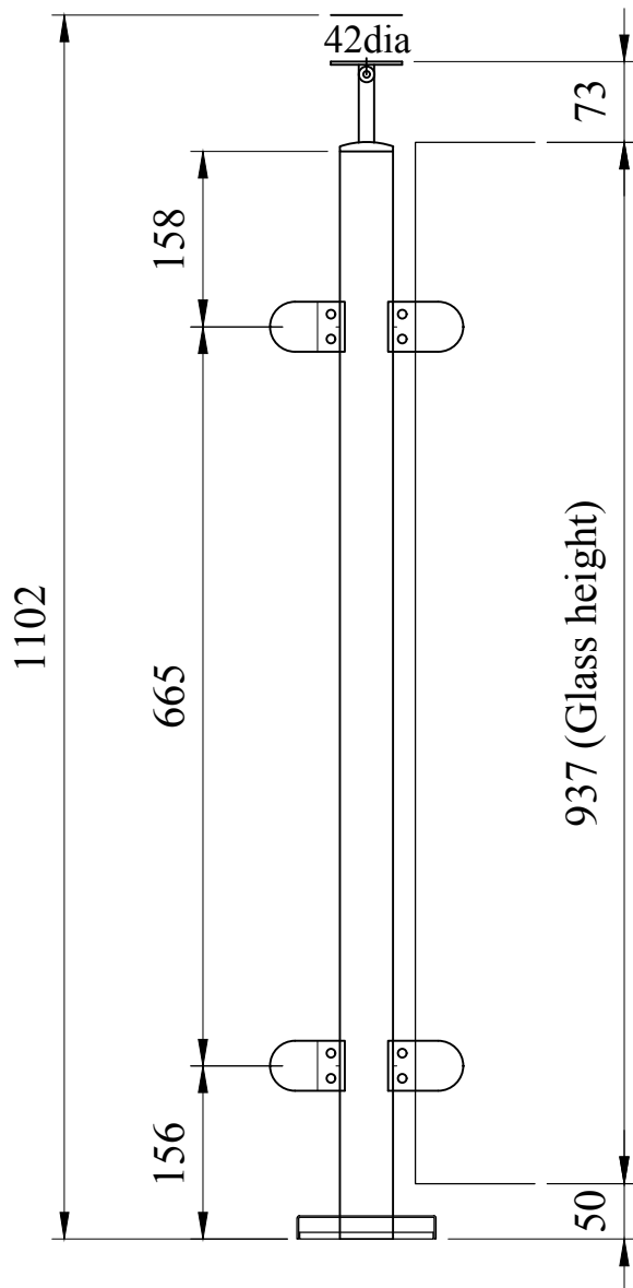
Middle Posts
