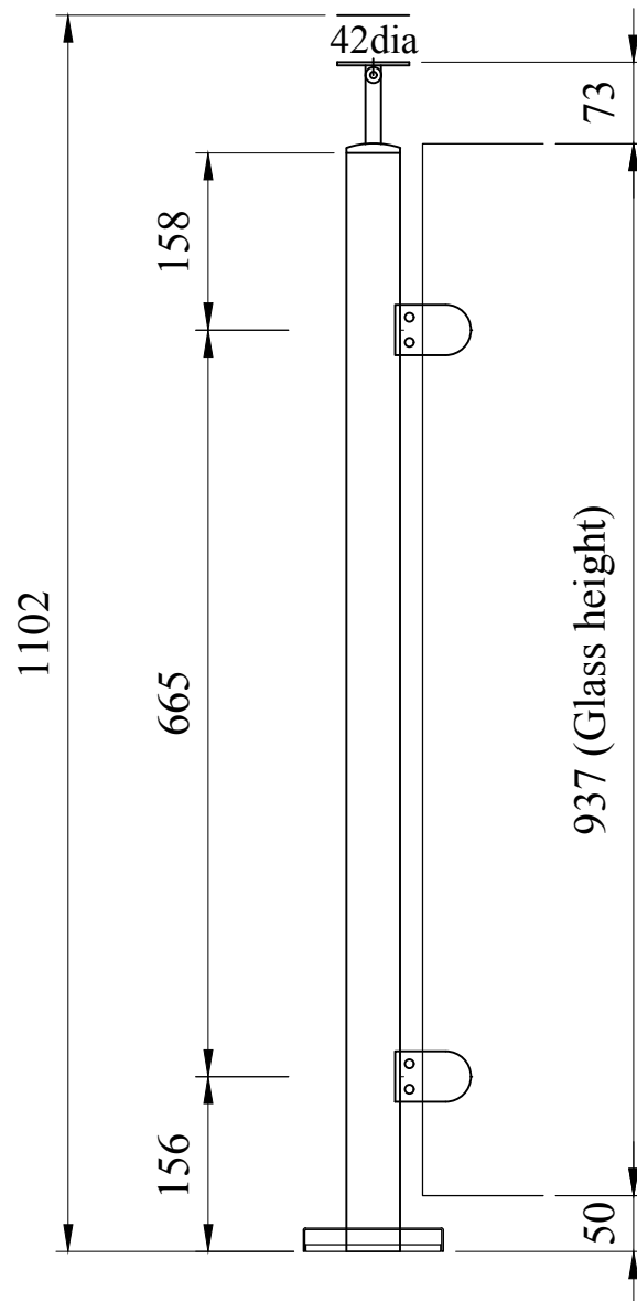
End Posts
